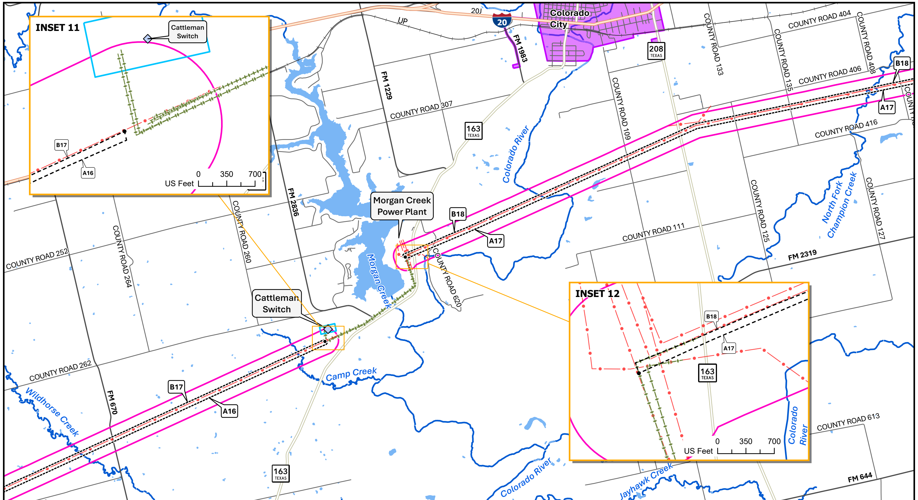
Figure 6 Detailed Route Description Map Consavvy Switch to Long Creek Switch 345 kV Transmission Line Rebuild Project Oncor Electric Delivery Company LLC Glasscock, Howard, Jones, Midland, Mitchell, Nolan, Shackelford, and Taylor Counties, Texas
