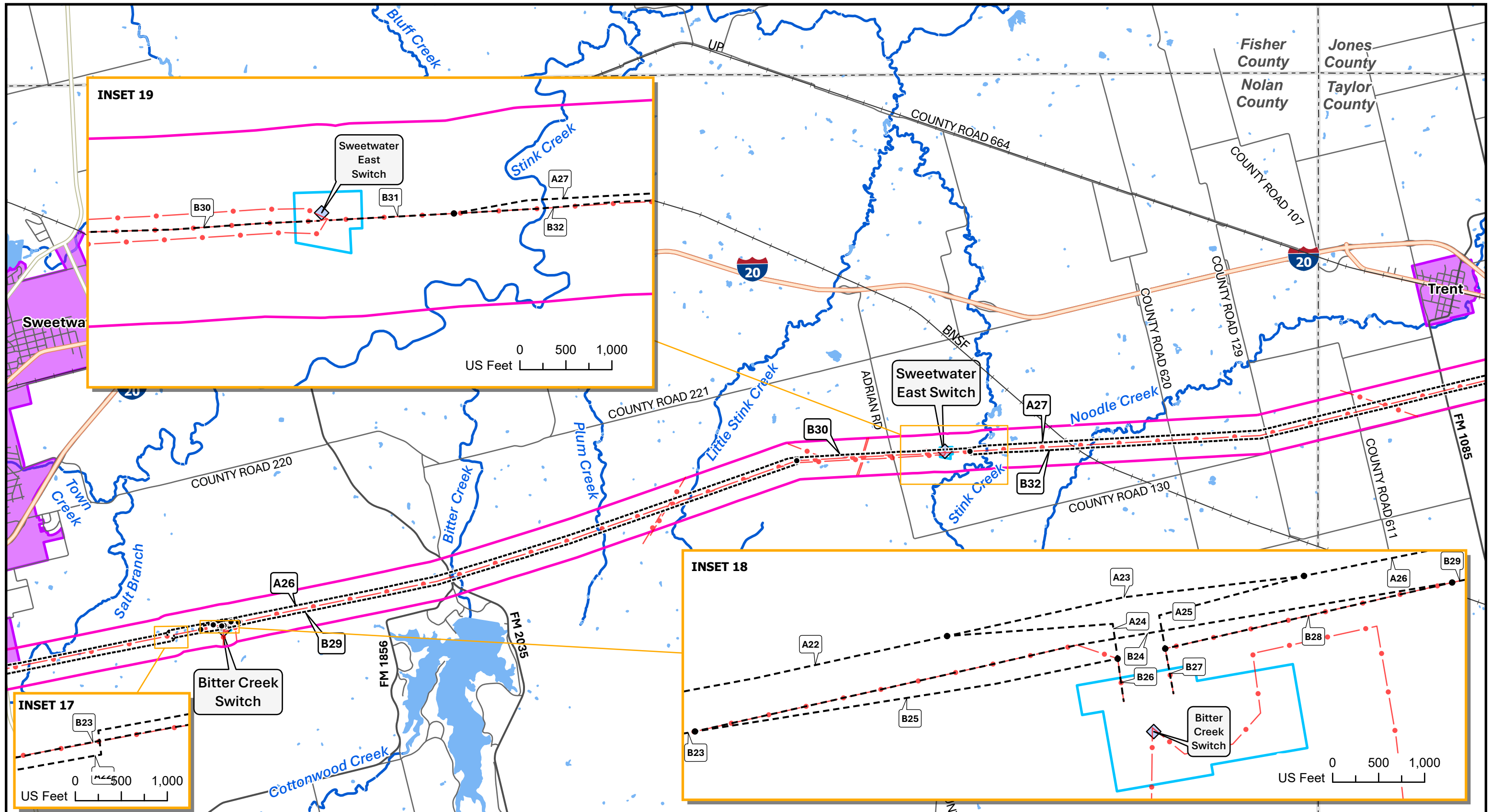
Figure 9 Detailed Route Description Map Consavvy Switch to Long Creek Switch 345 kV Transmission Line Rebuild Project Oncor Electric Delivery Company LLC Glasscock, Howard, Jones, Midland, Mitchell, Nolan, Shackleford, and Taylor Counties, Texas
