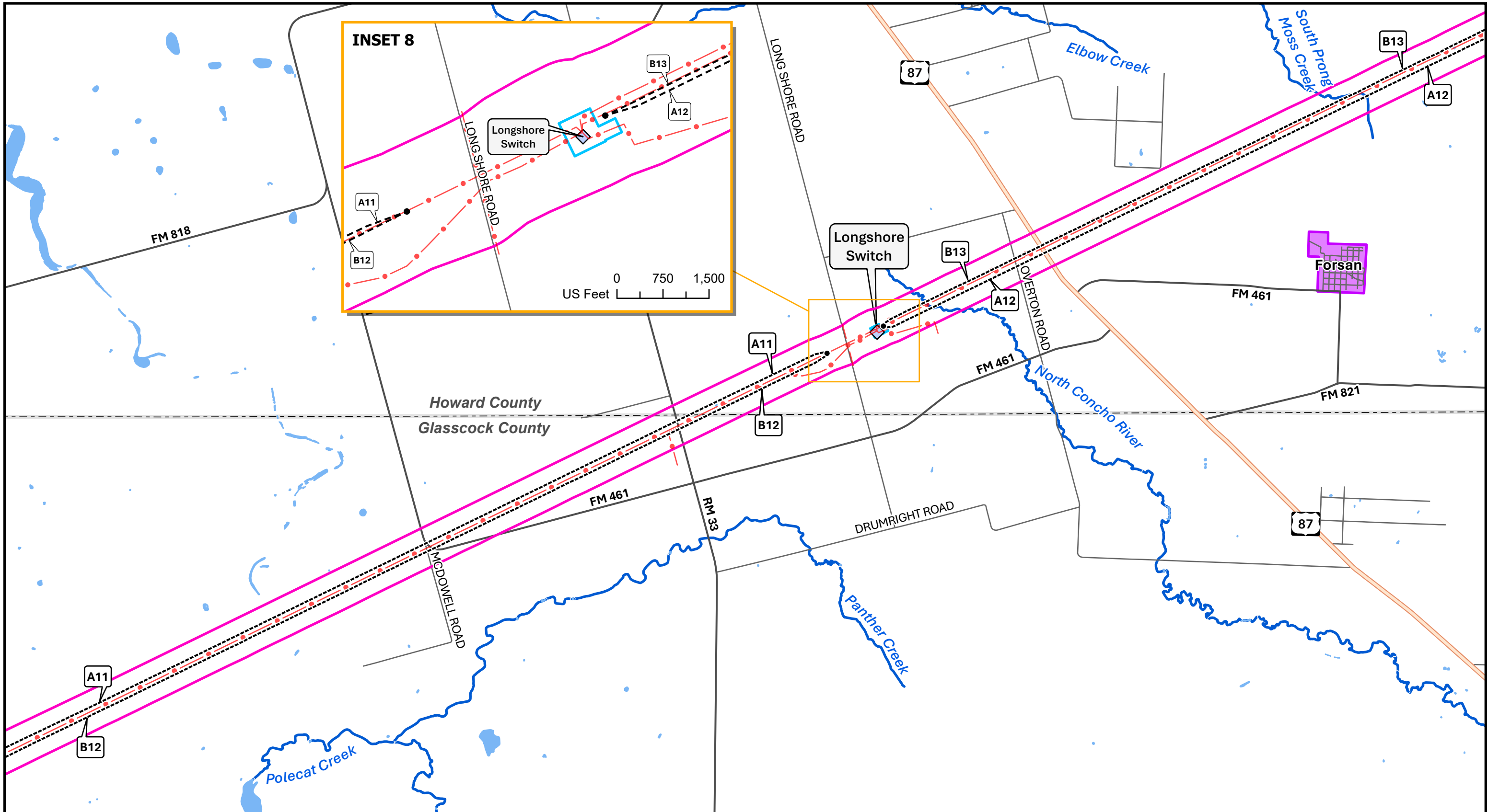
Figure 3 Detailed Route Description Map Consavvy Switch to Long Creek Switch 345 kV Transmission Line Rebuild Project Oncor Electric Delivery Company LLC Glasscock, Howard, Jones, Midland, Mitchell, Nolan, Shackelford, and Taylor Counties, Texas
