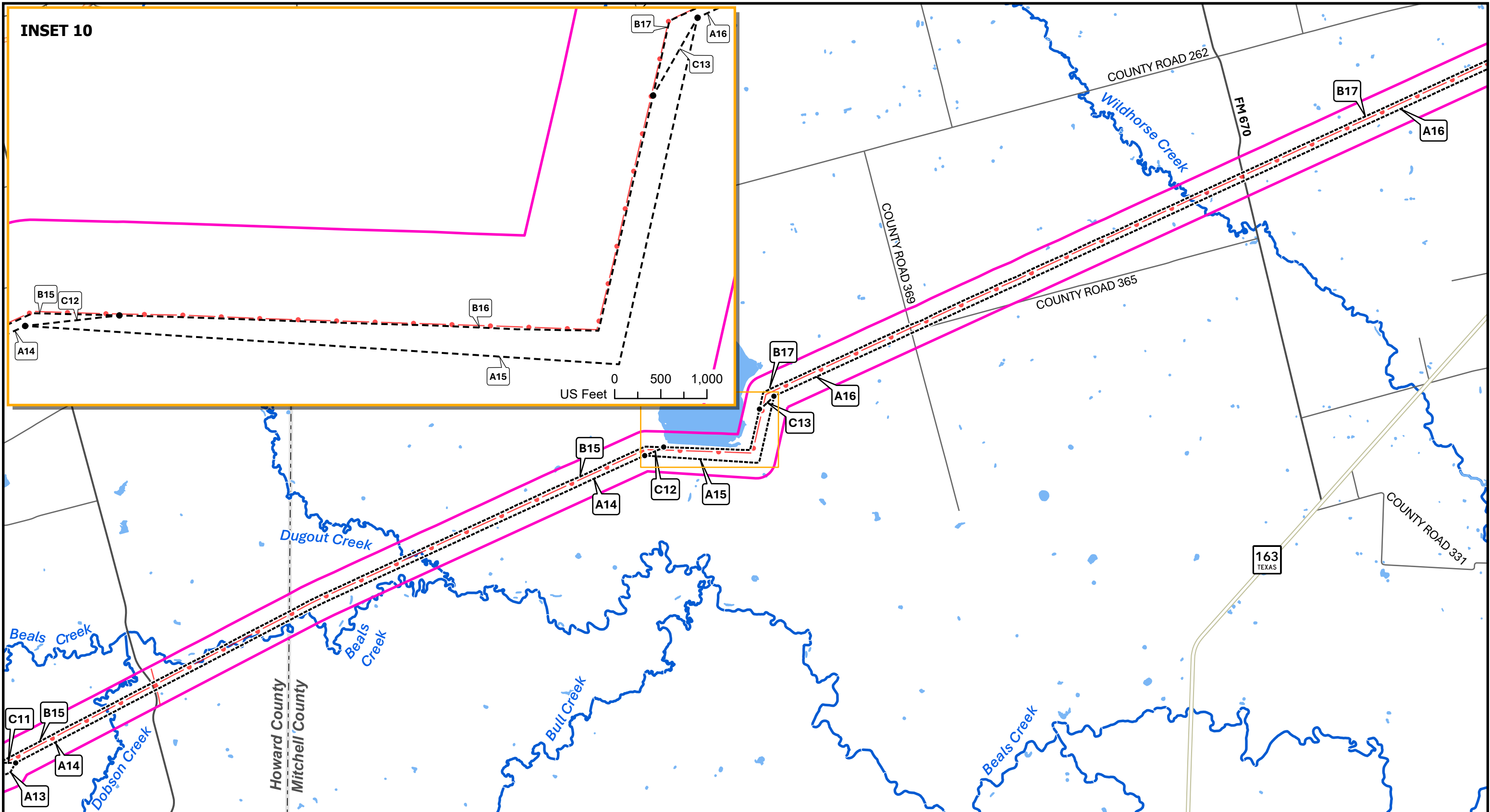
Figure 5 Detailed Route Description Map Consavvy Switch to Long Creek Switch 345 kV Transmission Line Rebuild Project Oncor Electric Delivery Company LLC Glasscock, Howard, Jones, Midland, Mitchell, Nolan, Shackelford, and Taylor Counties, Texas
