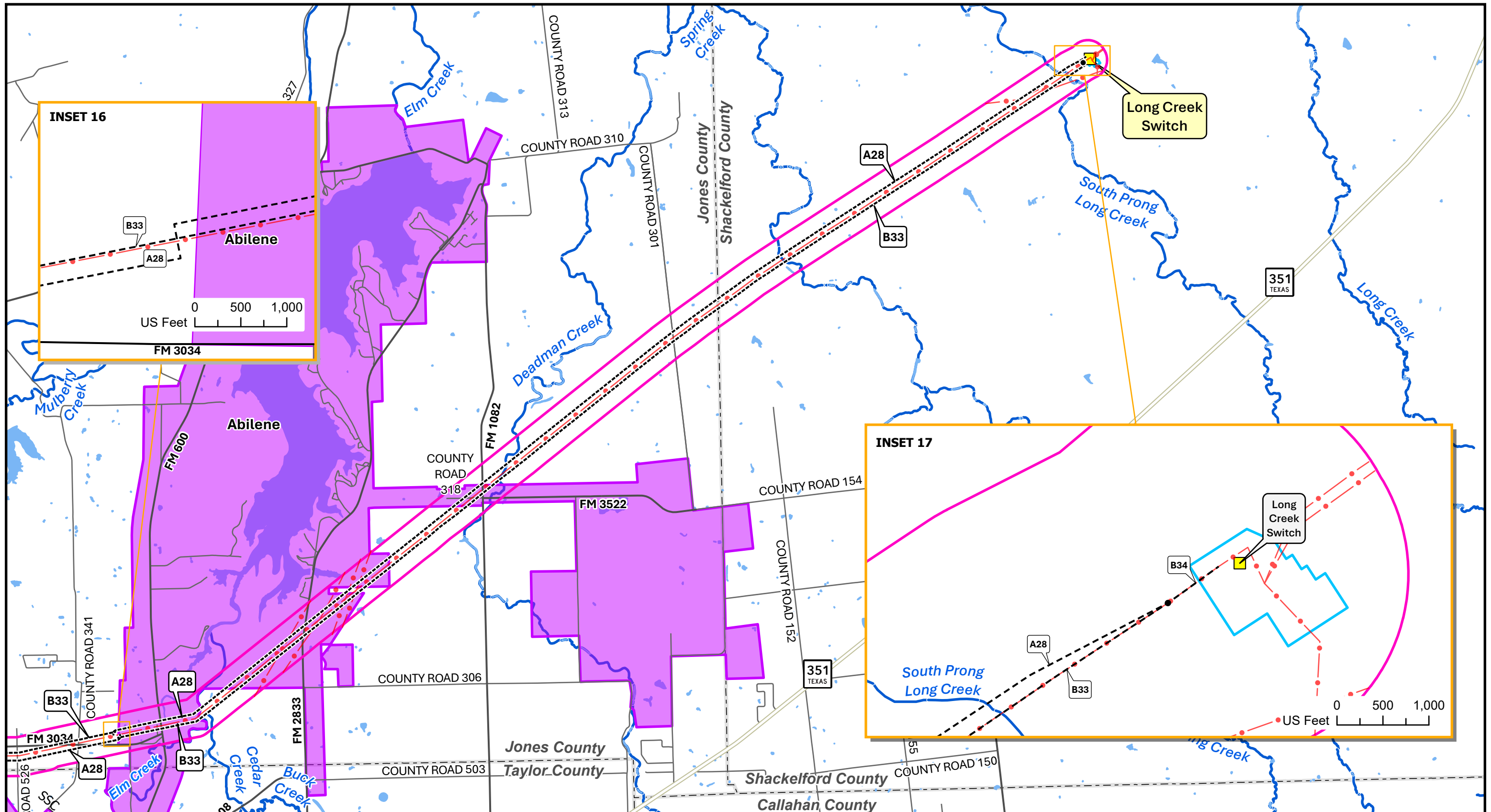
Figure 12 Detailed Route Description Map Consavvy Switch to Long Creek Switch 345 kV Transmission Line Rebuild Project Oncor Electric Delivery Company LLC Glasscock, Howard, Jones, Midland, Mitchell, Nolan, Shackelford, and Taylor Counties, Texas
