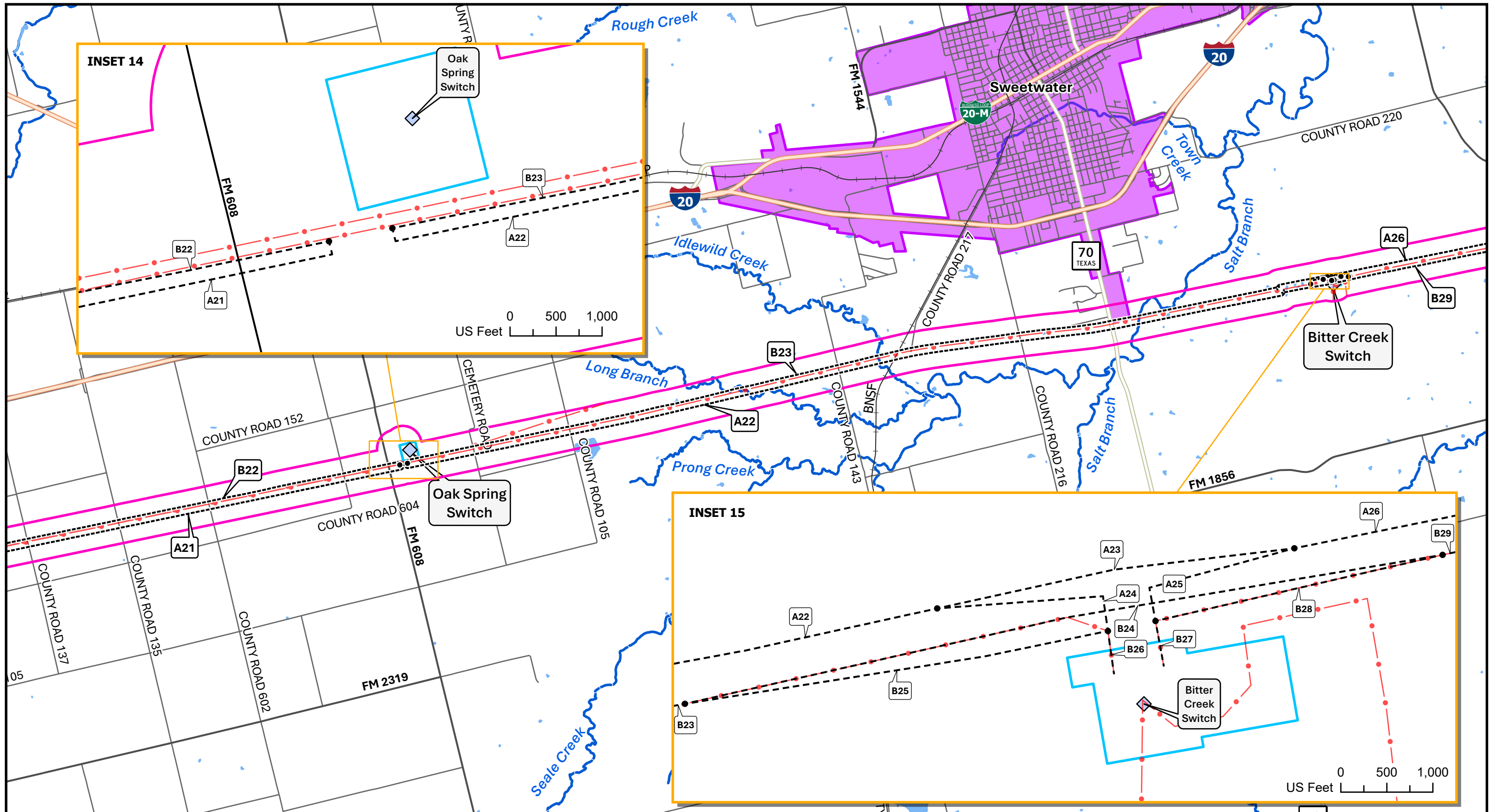
Figure 8 Detailed Route Description Map Consavvy Switch to Long Creek Switch 345 kV Transmission Line Rebuild Project Oncor Electric Delivery Company LLC Glasscock, Howard, Jones, Midland, Mitchell, Nolan, Shackelford, and Taylor Counties, Texas
