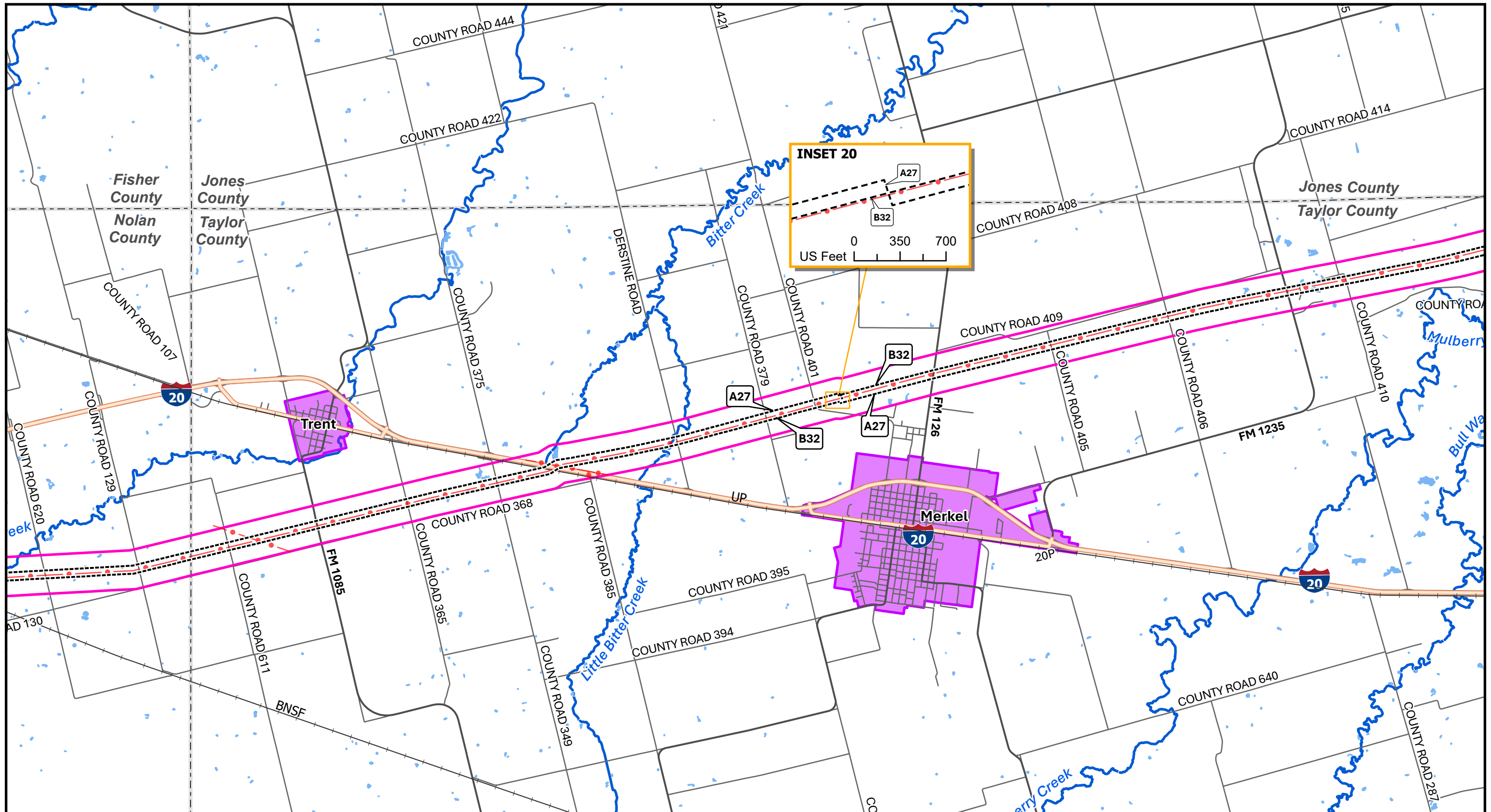
Figure 10 Detailed Route Description Map Consavvy Switch to Long Creek Switch 345 kV Transmission Line Rebuild Project Oncor Electric Delivery Company LLC Glasscock, Howard, Jones, Midland, Mitchell, Nolan, Shackelford, and Taylor Counties, Texas
