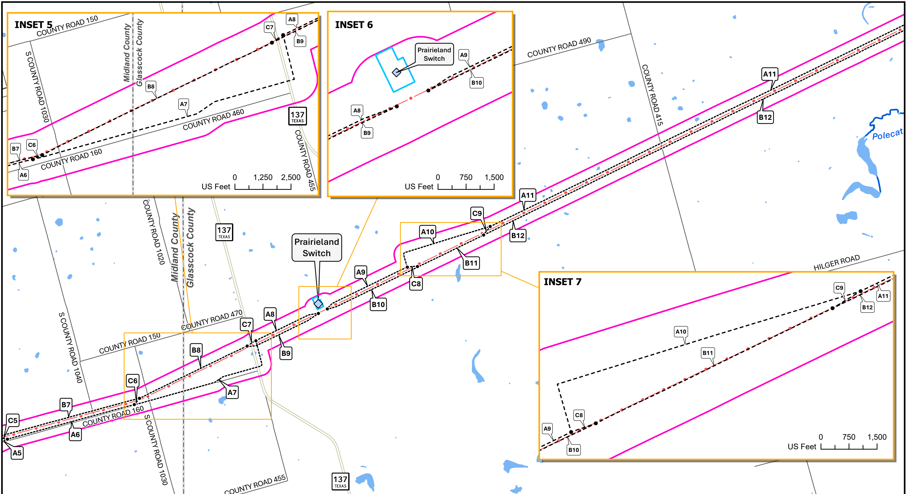
Figure 2 Detailed Route Description Map Consavvy Switch to Long Creek Switch 345 kV Transmission Line Rebuild Project Oncor Electric Delivery Company LLC Glasscock, Howard, Jones, Midland, Mitchell, Nolan, Shackleford, and Taylor Counties, Texas
