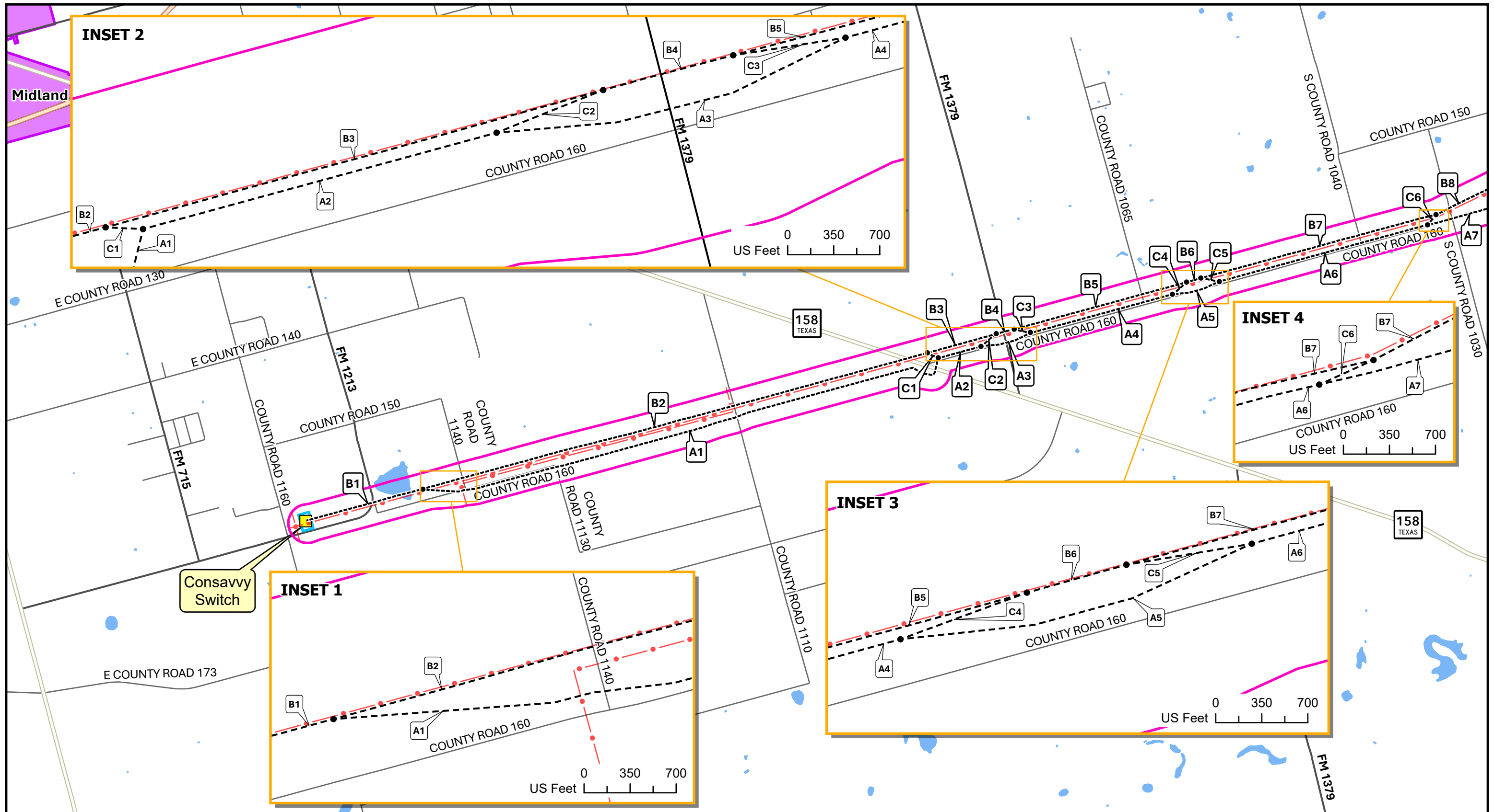
Figure 1 Detailed Route Description Map Consavvy Switch to Long Creek Switch 345 kV Transmission Line Rebuild Project Oncor Electric Delivery Company LLC Glasscock, Howard, Jones, Midland, Mitchell, Nolan, Shackleford, and Taylor Counties, Texas
