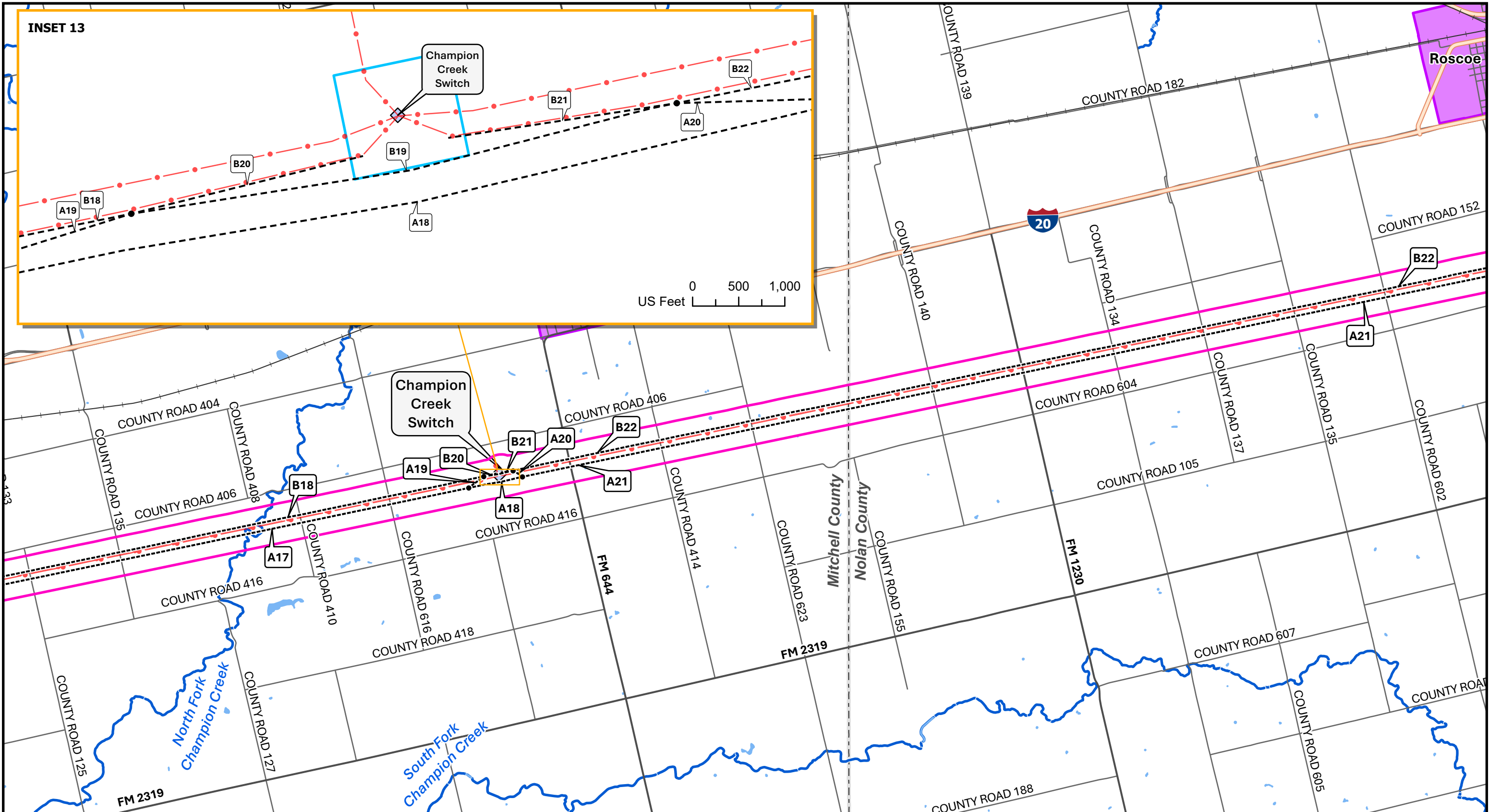
Figure 7 Detailed Route Description Map Consavvy Switch to Long Creek Switch 345 kV Transmission Line Rebuild Project Oncor Electric Delivery Company LLC Glasscock, Howard, Jones, Midland, Mitchell, Nolan, Shackelford, and Taylor Counties, Texas
